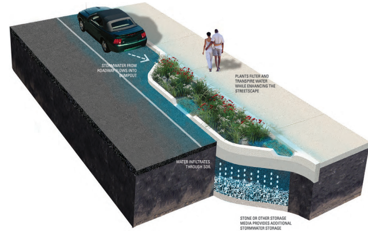
Mid-block Stormwater Bump-out
