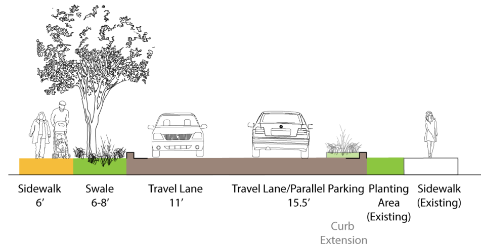
Example of a street that integrates planted swale and sidewalks within 50 ft right-of-way.
